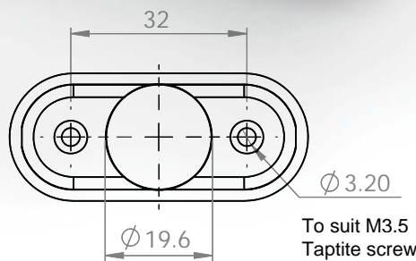
Rear Fix Cover
