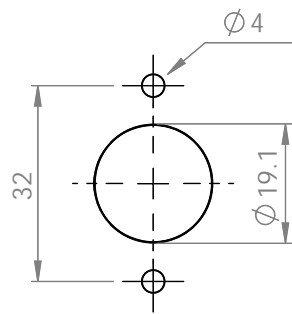
Fixing Details (rear fix only)
